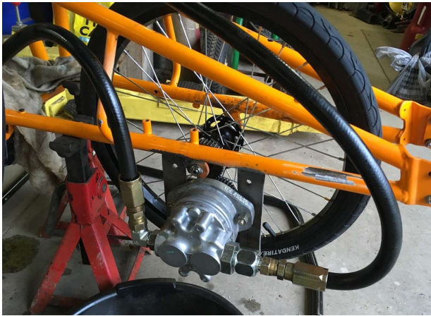
Photo 5: Test Rig
