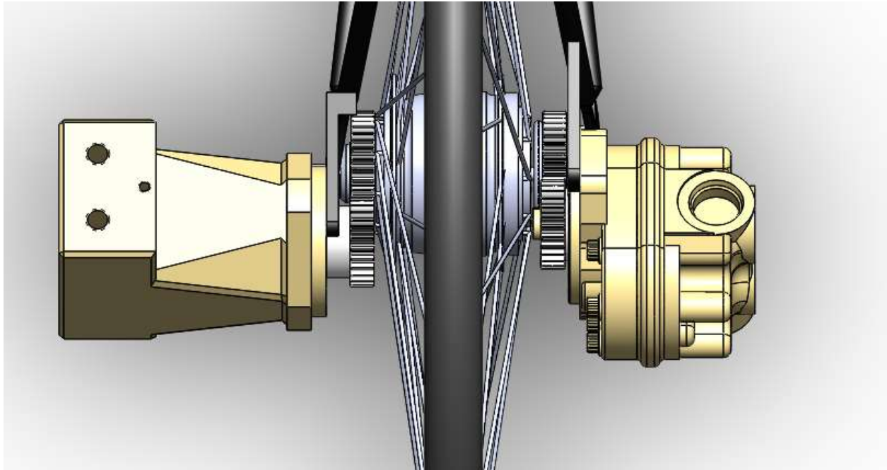
Close Up View 2: This view displays the gearing used on the rear hub and the motors. On the left is the Parker F11 motor used in the accumulation circuit. On the right is the Eaton 26 series motor. This view also shows the custom brackets being used to mount the motors.
